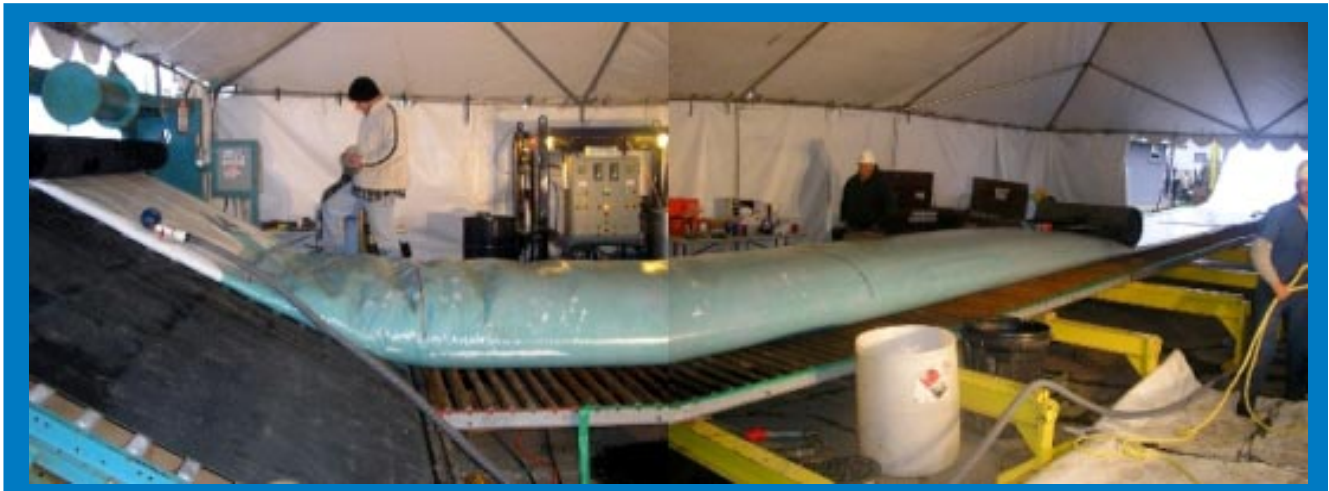
Felt tubing was impregnated inside a protective tent then conveyed out for inversion.
