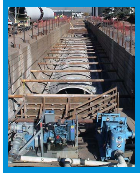
Five hundred feet of composite pipe were installed.
