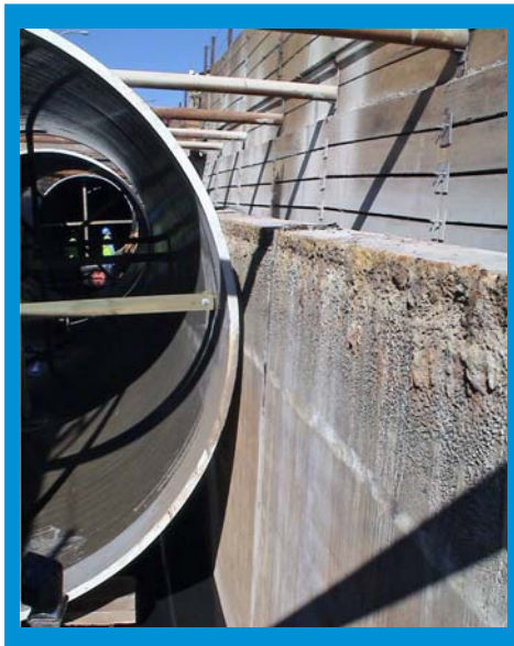
Belco custom-designed the pipe to fit precisely into the "trench" created by removing the damaged portion of the existing concrete culvert.
